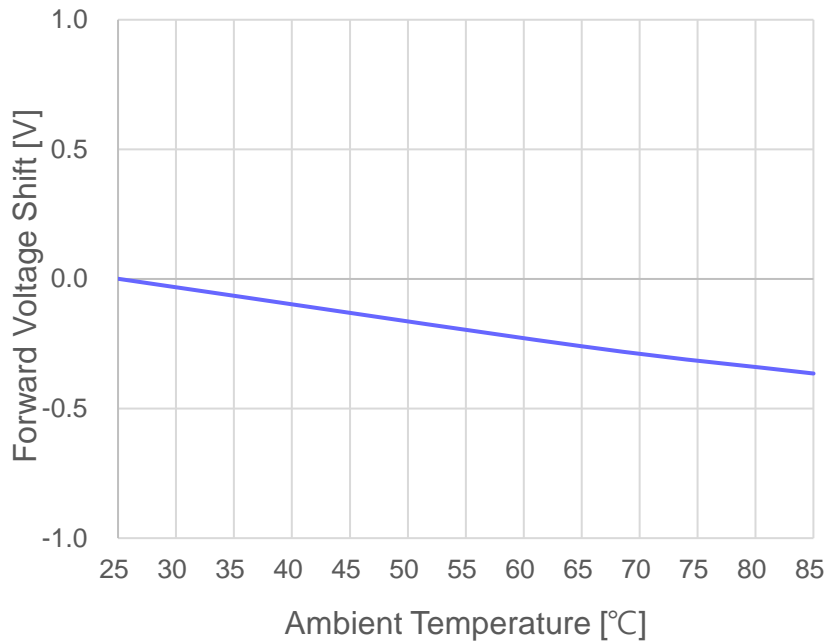
< Ambient Temperature vs. Forward Voltage Shift >
