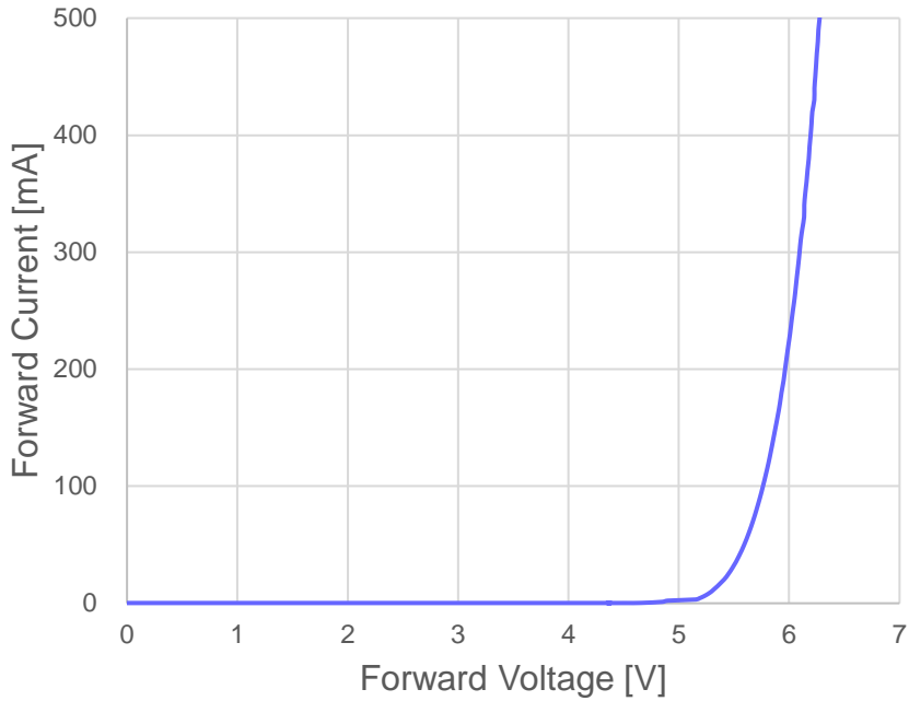
< Forward Voltage vs. Forward Current >
