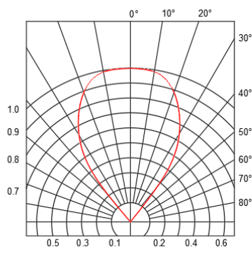
Fig.1 RADIATION DIAGRAM(A)
