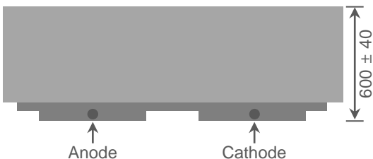
Cross Section
